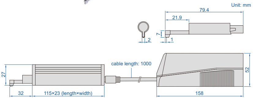
probe and main unit can be combined together
